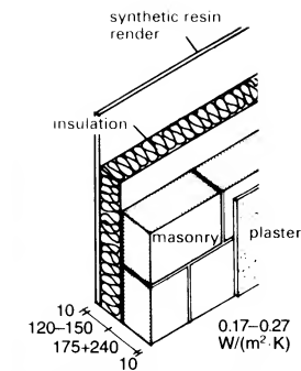
① Masonry with bonded insulation panels 0.17-0.27 W/(m 2 ·K)
